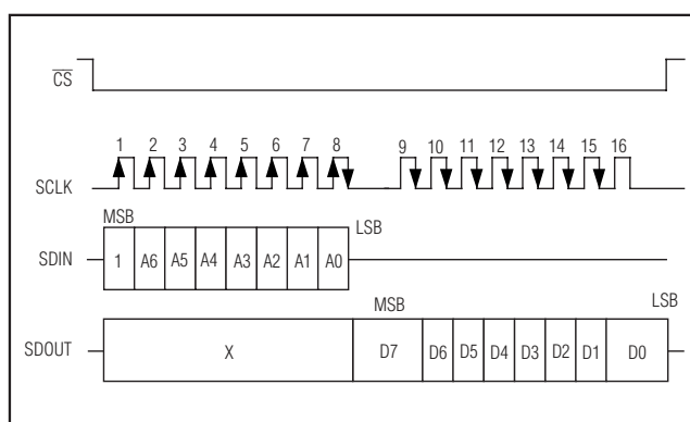
Figure 16. Read Operation
