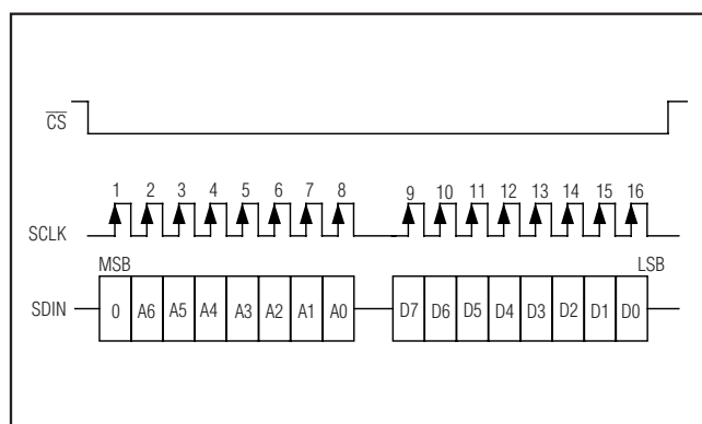
Figure 15. Write Operation
